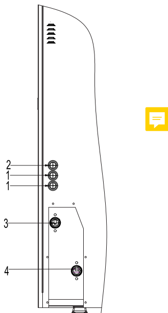
Figure 3-4.2.3: Wiring hole for 12/16 kW models
